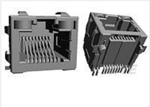
TE 产品编号6339191-1 MJ,RJ45,SMT,SHLD,LED (Y/G)
