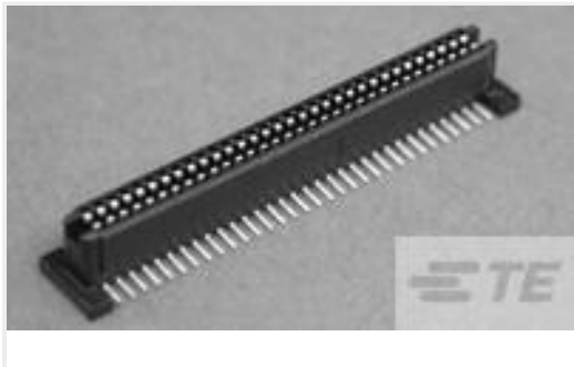
TE 产品编号5146893-1 1FHR,64,30A/S,S,C,S08,09,10
