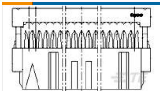
TE 零件编号2-215911-0 20 WAY GREY MK II RECP
