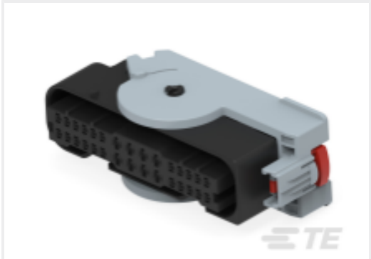
TE 产品编号7-2109446-2 MCP 1.5/2.8 SLD 30P PLUG ASSY
