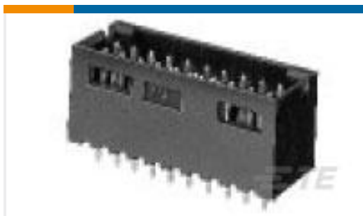
TE 产品编号5-102618-4 12 MODII HDR DRST SHRD .100CL
