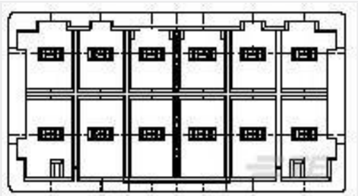
TE 产品编号2-1871571-3 GIC 3.3 HEADER ASSY 12POS
