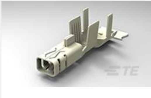
TE 产品编号1971785-1 PTL RECEPTACLE CONTACT, 20 - 24 AWG
