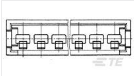
TE 产品编号280630 AMPMODU II COSI PIN HSG, SGL ROW, 6 POS.
