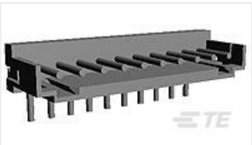
TE 产品编号292253-9 CT CONN MT HDR ASSY H 9P NAT
