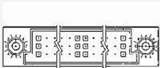
TE 产品编号532433-8 HDI PIN ASSY 3 ROW 165 POS
