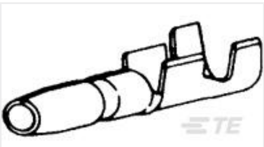
TE 产品编号61388-1 SHUR PLUG 156 20-16 AWG PTPBR
