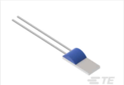
TE 产品编号NB-PTCO-168 Pt1000, 2.0x5.0, Class A, PTFD102A1G0
