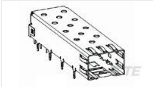
TE 产品编号2227303-3 CAGE ASSEMBLY, SFP, .071 TAIL
