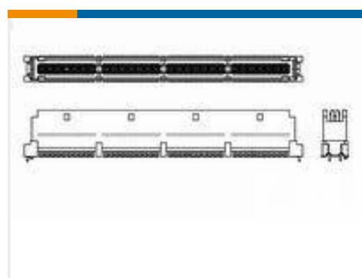
TE 产品编号2069399-2 V-P ASSY 16MM 160P IEX 0.8MM H-SP CONN.
