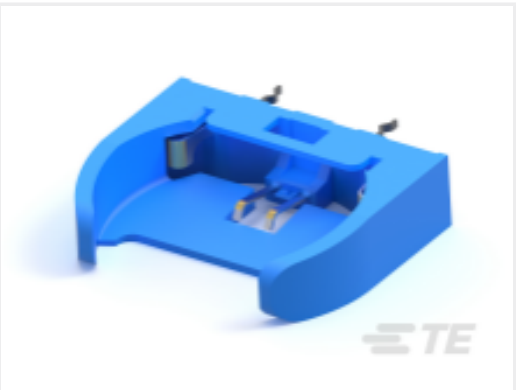
TE 产品编号 1775485-2 Battery Holder, 3.6mm, BLU,low profile
