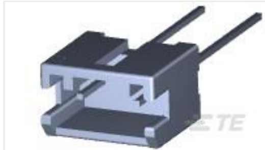
TE 产品编号5-1376500-2 2.5 SMC HDR 2(3)POS WHITE TAPE
