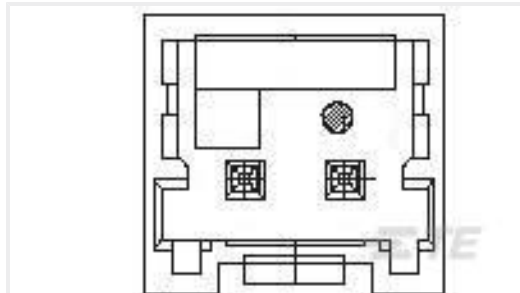
TE 产品编号1971032-2 2POS HEADER ASSEMBLY FOR GIC 2.0 EV
