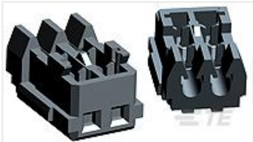
TE 产品编号2-353293-7 1.5MM CT MT REC ASS'Y 7P BLACK
