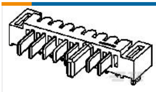
TE 产品编号1932154-1 2mm pitch Battery Plug Assy.7Pos Reverse
