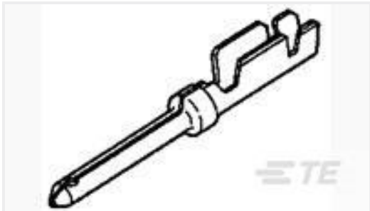
TE 产品编号1658670-5 CONT,PIN,PLATED,22DF,LP,#22-28, SM-PAK
