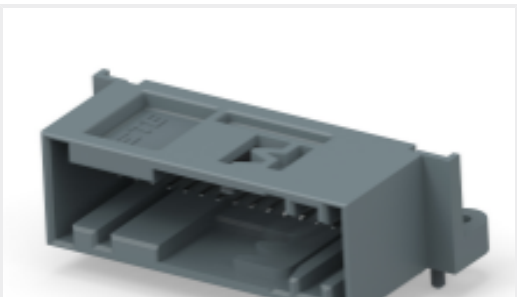
TE 产品编号2393361-1 32POS,TAB0.63X0.63,HDR ASSY, 90DEG,SLDR
