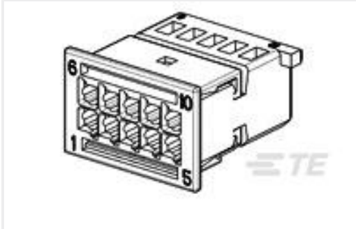
TE 产品编号1-968636-2 10POS MQS REC COD A
