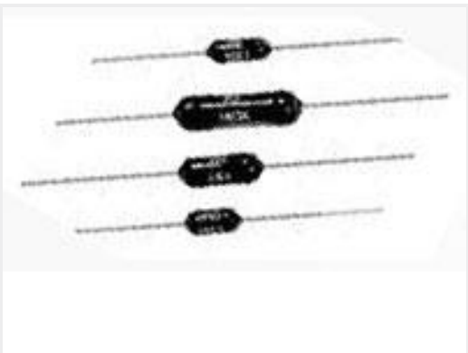
TE 产品编号7-1879682-8 H8 63R4 0.1% 50PPM
