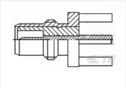
TE 产品编号1-1337485-0 SMC JACK STR PCB THRU HOLE 50 OHM GOLD
