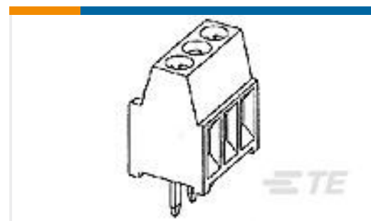
TE 产品编号282834-6 TERMI-BLOK PCB MOUNT, 90 6P.
