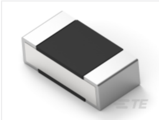
TE 产品编号2176304-1 RP 1E 0.1W 10R 0.1% 25PPM 5K RL
