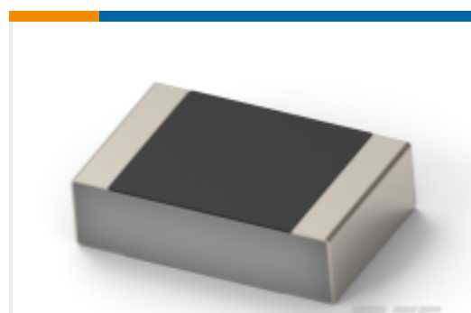
TE 产品编号2176453-7 CPF 0201 6K65 0.1% 25ppm 1K RL
