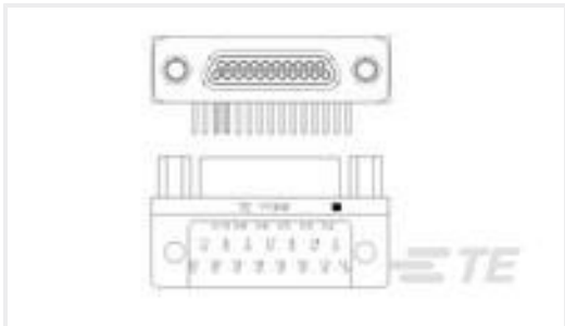
TE 产品编号1-1532252-1 M83513/10-C03NN = MCKS-N1-B-21PRT1B
