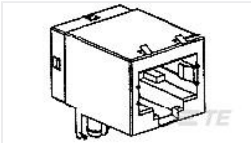
TE 产品编号5558344-1 MJ,8POS,R/A,CAT5,SHLD,PNL GND
