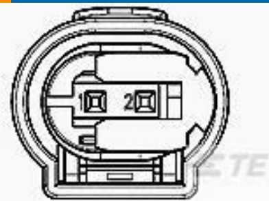
TE 产品编号284703-1 2POS MQS REC SEALED COD A
