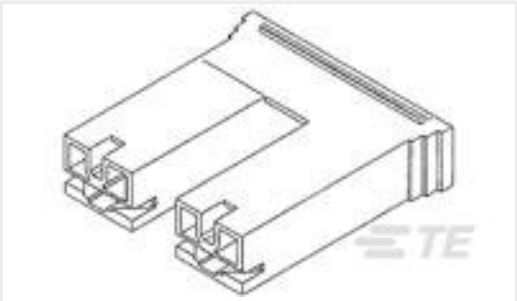
TE 产品编号520935-6 PL&STANDARD FASTON 250 HSG REC YELLOW
