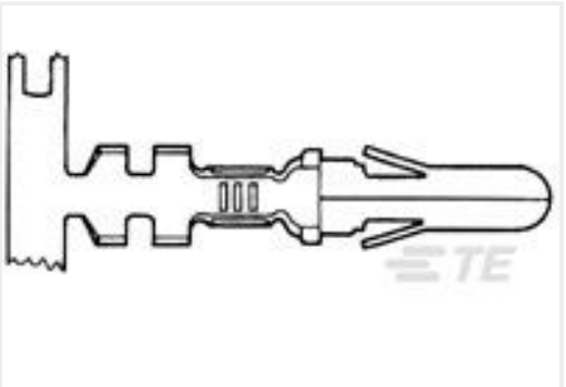
TE 产品编号350201-2 .140 DIA PIN 14-10 PTPPHBZ
