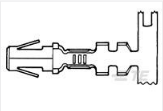
TE 产品编号350200-2 .140 DIA SOK 14-10 PTPPHBZ
