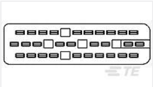
TE 产品编号963222-1 SEALING F/29P HSG
