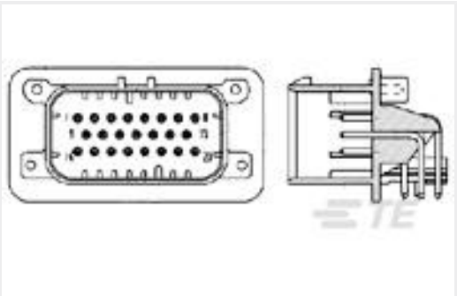
TE 产品编号1-776087-4 23POS,PIN DIA 1.3,HDR ASSY,90DEG, COD 4
