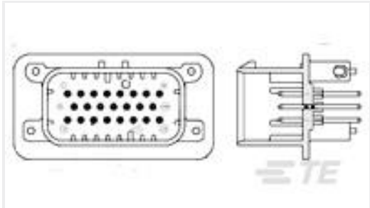
TE 产品编号1-776228-1 23POS,PIN DIA 1.3,HDR ASSY, 180DEG,COD 1
