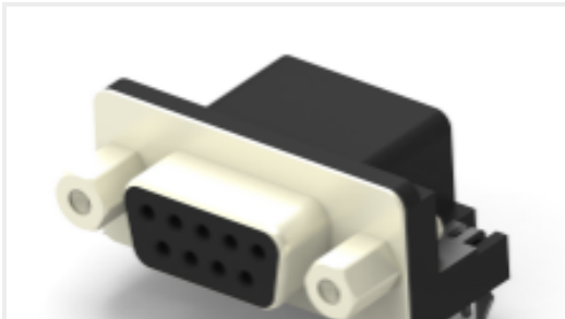
TE 产品编号2301844-2 AMPL REC HD20, R/A, 9P, B/L,4-40 S /LOCK
