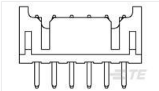
TE 产品编号1-1470109-0 2.0mm Pitch Header,Dip 10p
