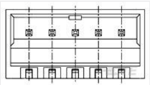
TE 产品编号5-1775444-5 EMIX CONN., 1.5MM PITCH, HDR, R /A, 5P
