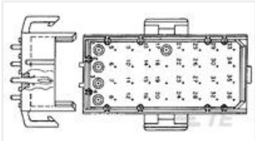
TE 产品编号640499-1 04P MR HDR ASSY V0
