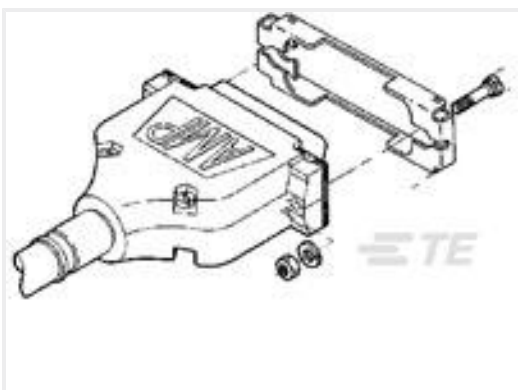
TE 产品编号5745584-1 UNIV SLIDLTCH KIT SZ 3
