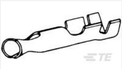
TE 产品编号42428-5 PIN TERMINAL RECEPTACLE 24-20 AWG TPPHBZ
