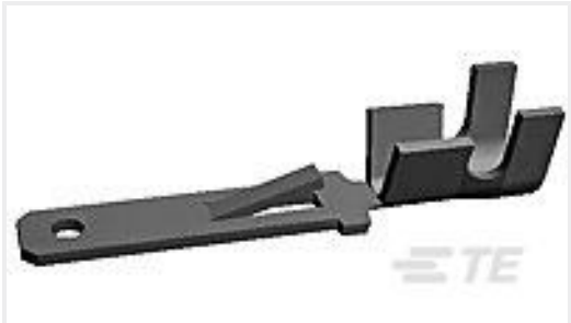
TE 产品编号160457-2 FF 250 TAB 18-14AWG TPPB
