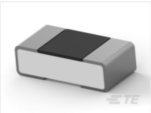
TE 产品编号5-2176364-8 RQ 0402 18K2 0.1% 10PPM 5K RL
