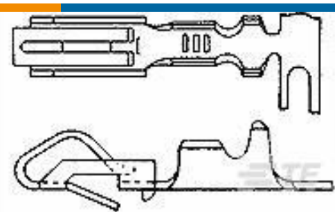
TE 产品编号350011-3 BIF-LEAF CONT PTPPHBZ LP 24-18
