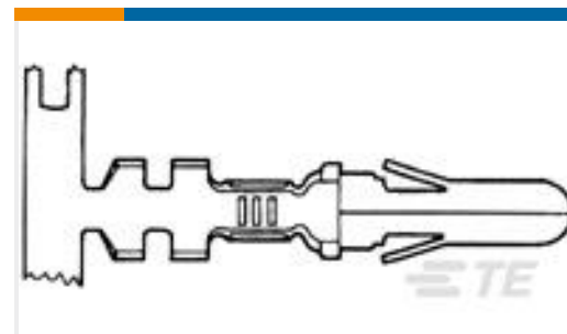
TE 产品编号350389-1 .140 DIA PIN 20-14 PTPBR L/P
