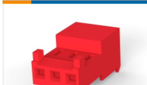
TE 产品编号3-643815-3 Nylon Tin Plated Receptacle: 2.54 mm, with Mating Alignment, MTA 100
