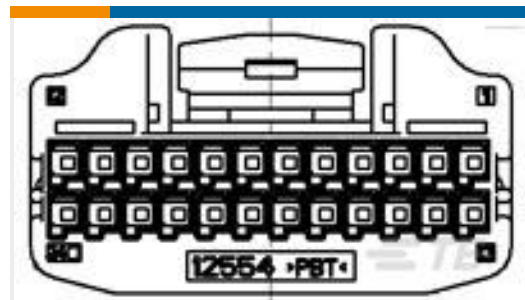
TE 产品编号1717118-1 0.64 III 32POS PLUG ASSY
