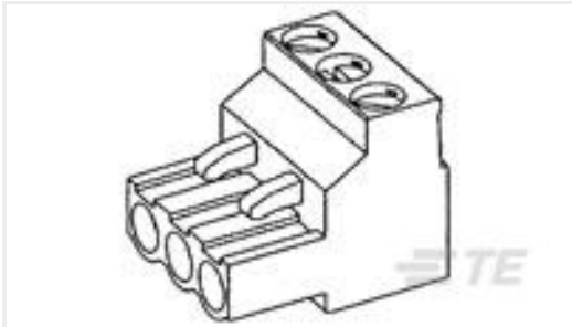
TE 产品编号796634-2 2 POS 5.08MM R/A PLUG,TRM BLK
