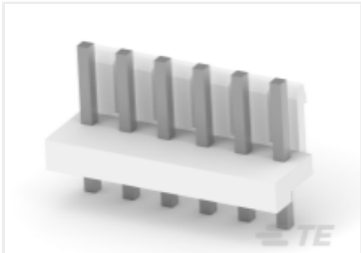
TE 产品编号 1-1612911-6 3.96/7.92 EP CONN. HDR ASS'Y 6/10P
