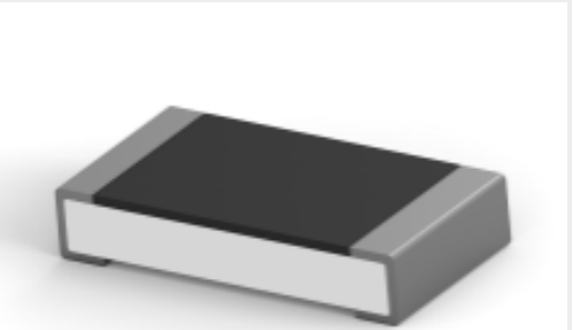
TE 产品编号5-2176388-8 RQ 1206 39R2 0.1% 10PPM 5K RL
