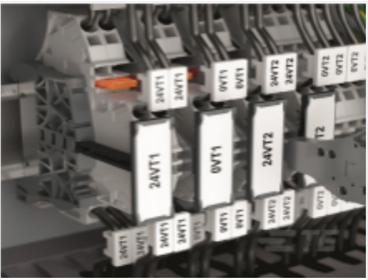
TE 产品编号1SNK900630R0000 MCLH
