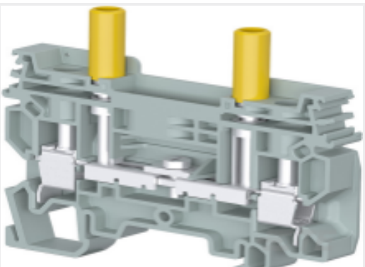
TE 产品编号1SNL608311R0000 C6/8.ST1.IP20
