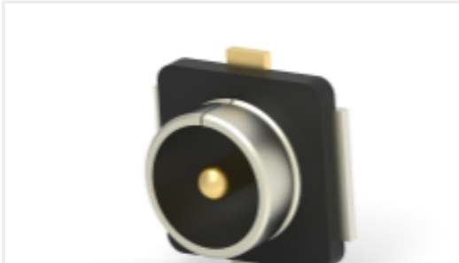
TE 产品编号2337019-1 UMCC Micro-Coax receptacle, Gen 1
